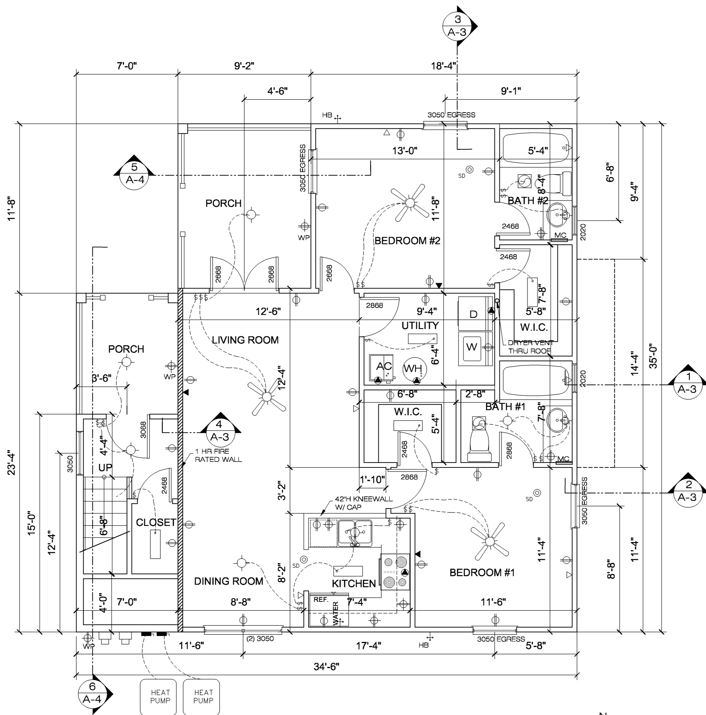
BUILDING #1 - FIRST FLOOR PLAN W/ ELECTRICAL
