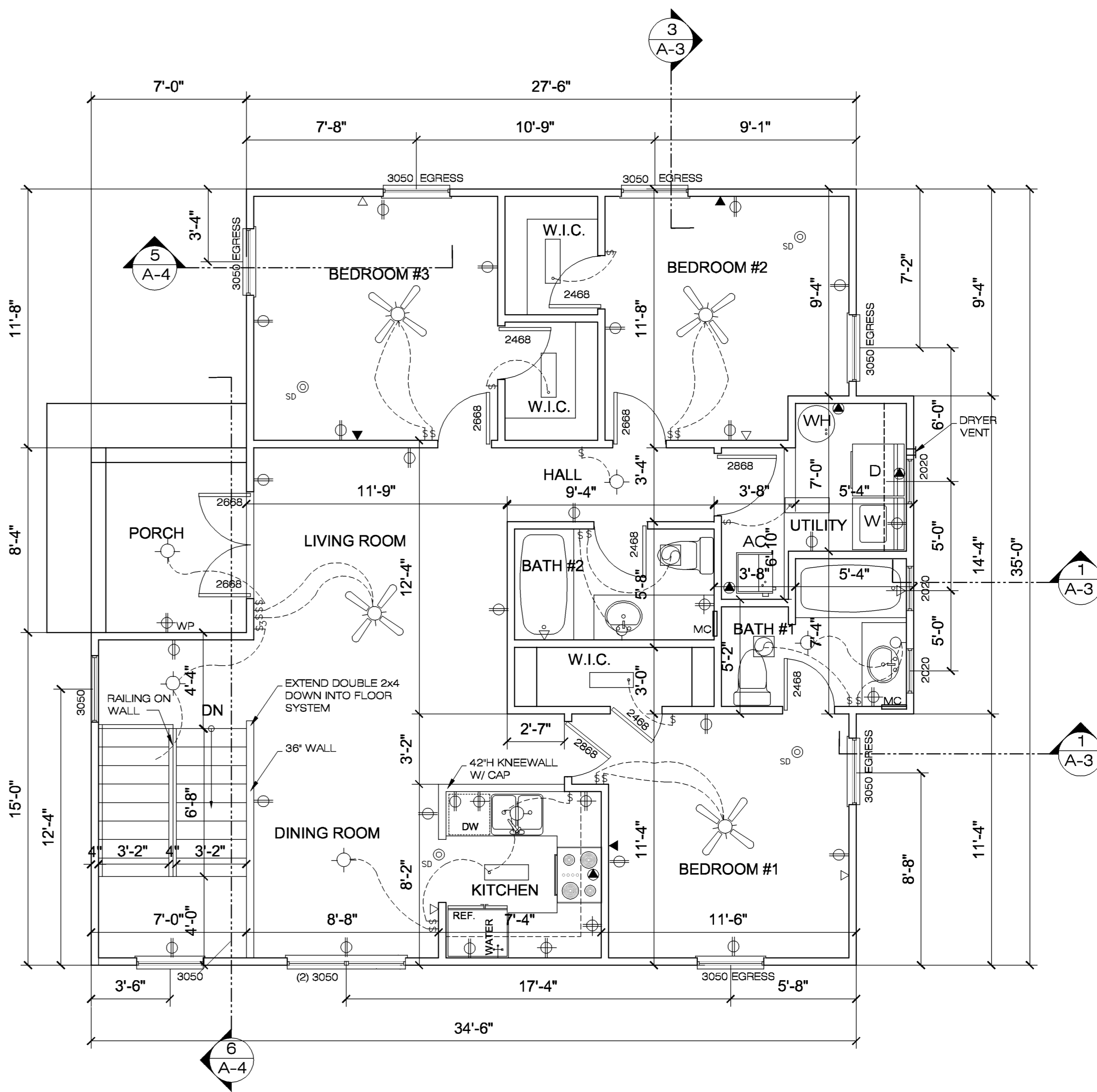
BUILDING #1 - SECOND FLOOR PLAN W/ ELECTRICAL
